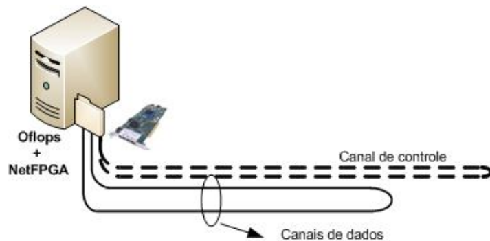
Figura 4.10 - Setup Loopback Oflops.
