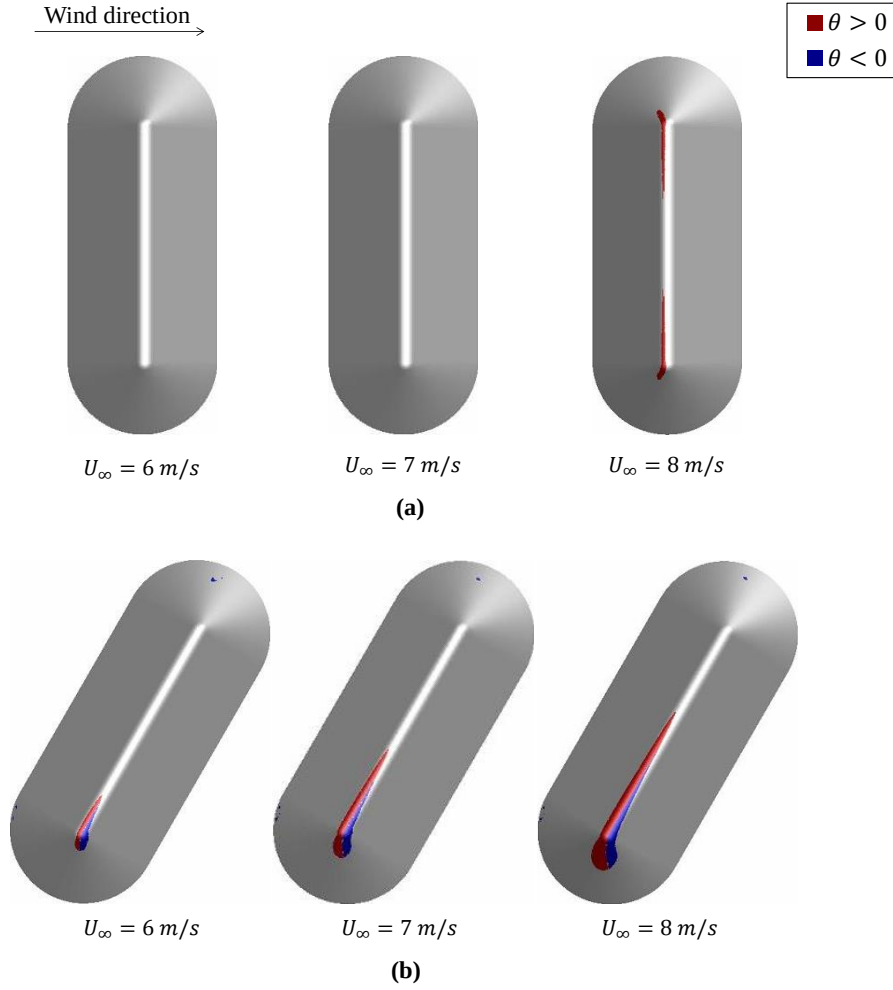
Figure 3.8: Areas on the pile surface where the black particles become erodible for the orientations of (a) 90° and (b) 60°
