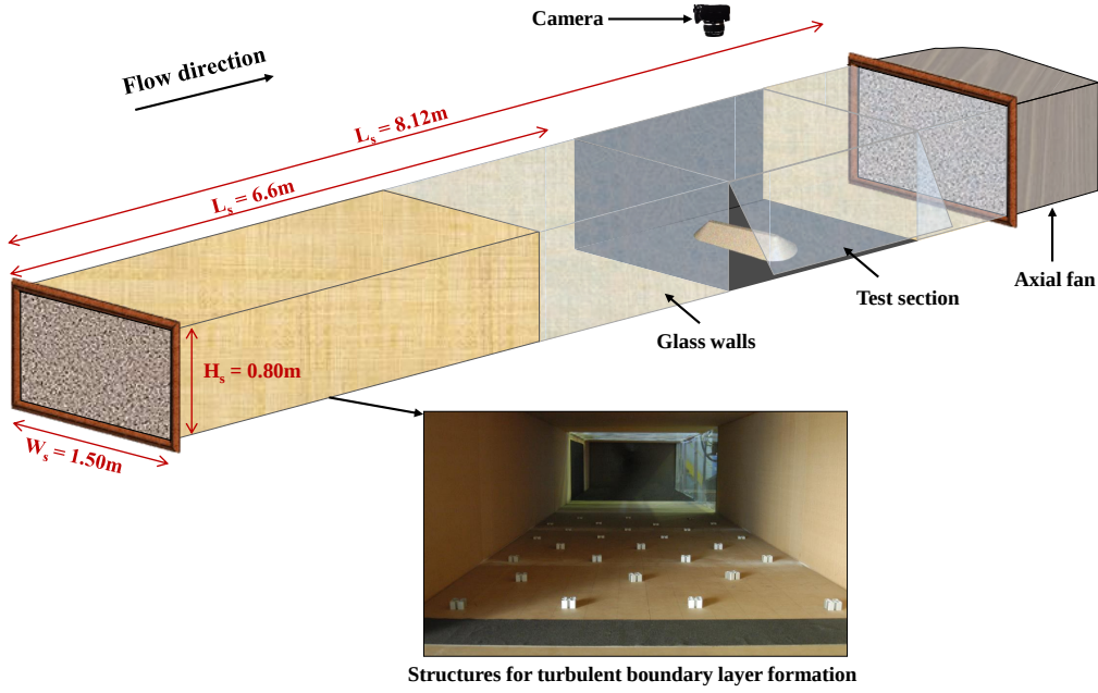
Figure 1: Wind tunnel scheme
