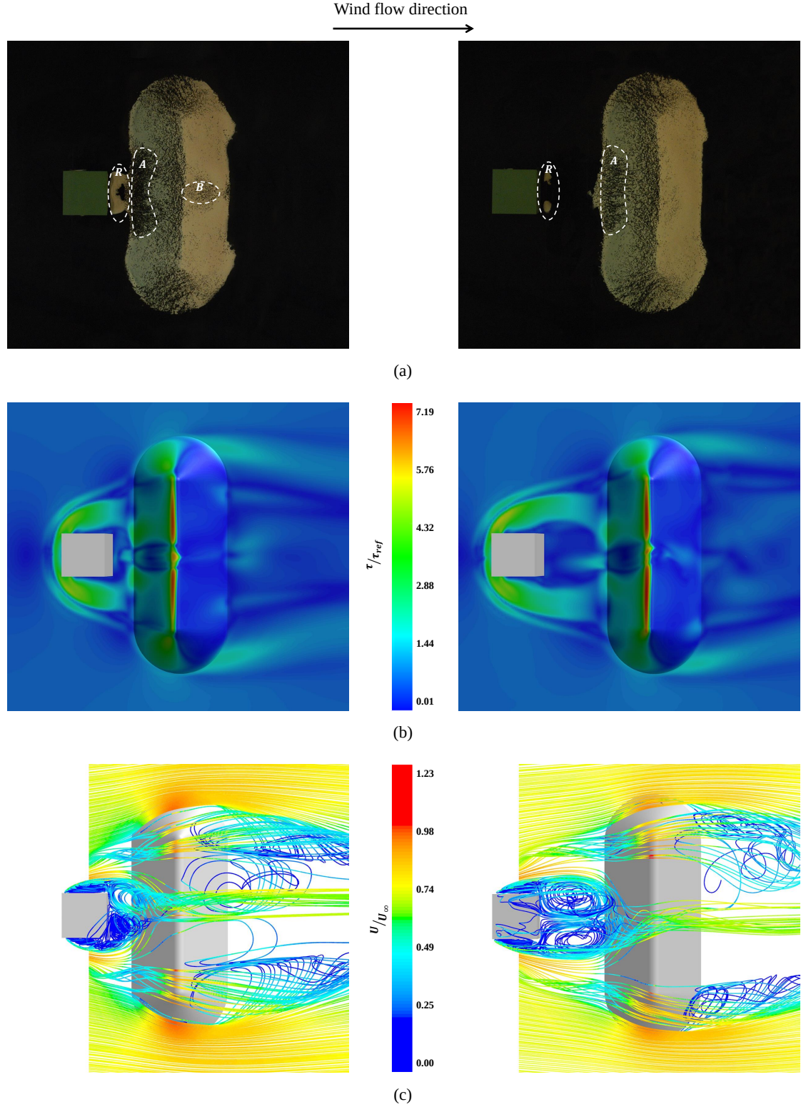
Figure 3.1: Experimental and numerical results for a stockpile downstream a cubic building with the face perpendicular to the flow, separated by gaps 0.5H_b and 1.5H_b : (a) Photograph of the top view of the eroded sand stockpile after pavement, (b) Wall shear stress distribution on the pile surface and on the ground and (c) Pathlines of the flow over the pile
