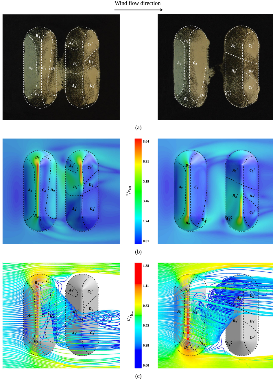
Figure 7: Experimental and numerical results for two parallel stockpiles oriented 90° separated by 0.9h and 1.8h gaps: (a) Top view of the eroded sand stockpiles after the pavement phenomenon, (b) Mean wall shear stress on the pile surfaces and on the ground and (c) Mean flow pathlines over the piles. Four wind erosion regions are highlighted on each pile, according to the degree of wind exposure: zones A_2 , B_2 , C_2 and D_2 in the upstream pile (pile p_2 ) and zones A'_2 , B'_2 , C'_2 and D'_2 in the downstream pile (pile p'_2 ).
