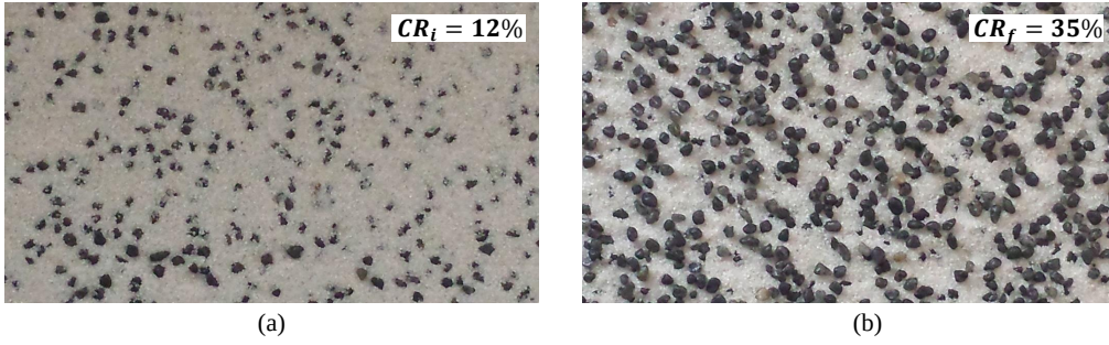
Figure 10: Pictures of the sand bed (a) before and (b) after the pavement for U_\infty = 8.5 m/s with \alpha_{NE} = 20\%
