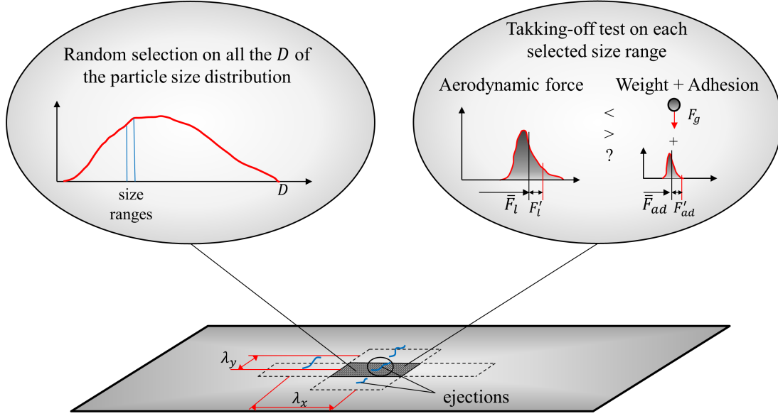
Figure 1.11: Principle of the model (Descamps, 2004)
