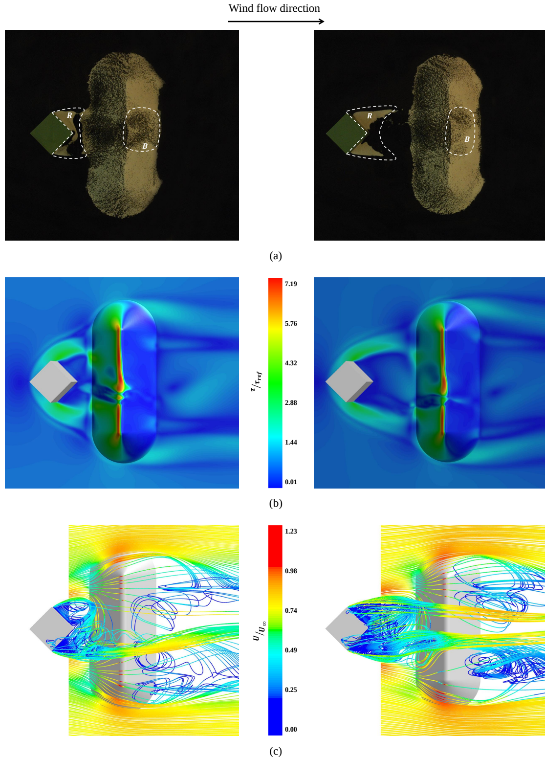
Figure 3.2: Experimental and numerical results for a stockpile downstream a cubic building oriented 45^\circ to the main flow, separated by gaps 0.5H_b and 1.5H_b : (a) Photograph of the eroded sand stockpile after pavement, (b) Wall shear stress distribution on the pile surface and on the ground and (c) Pathlines of the flow over the pile
