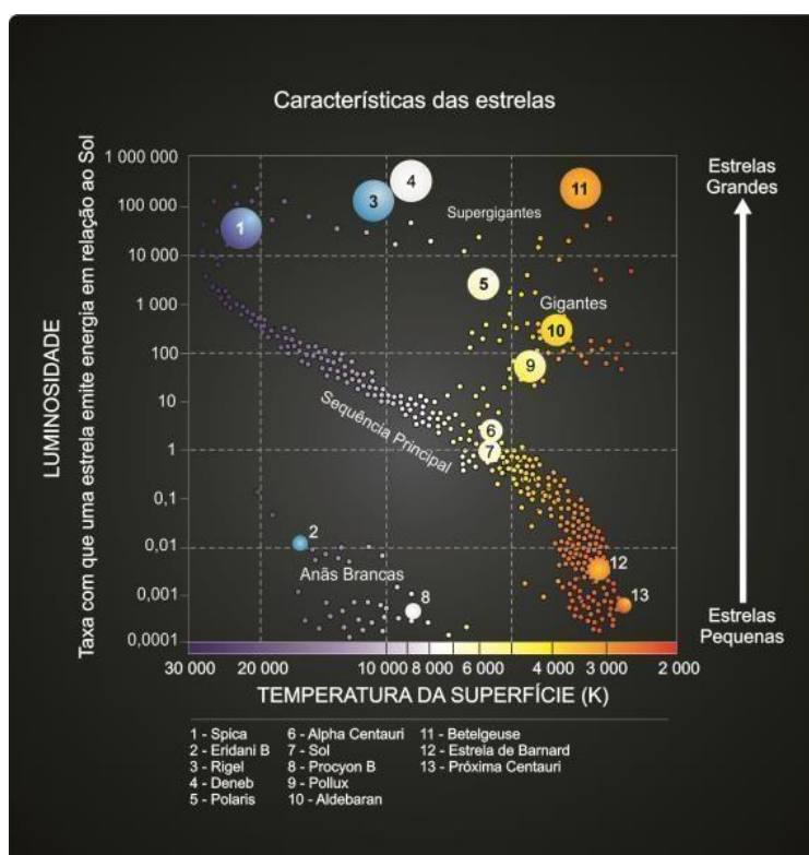
Figura 08 – Diagrama H-R
