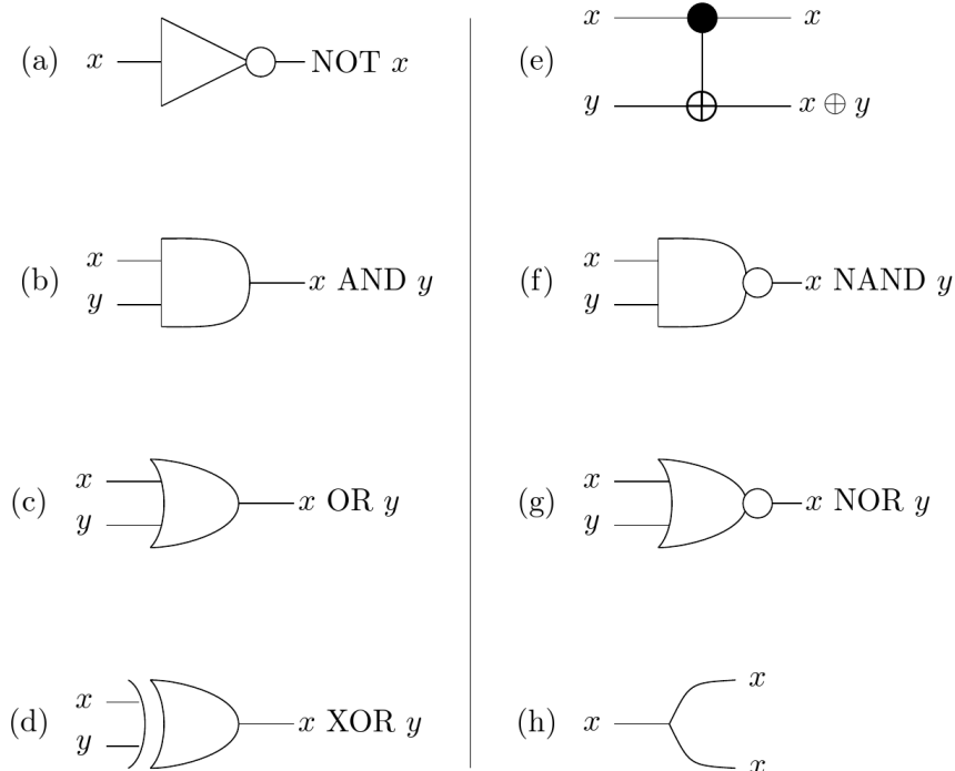
Figura 9 – Alguns exemplos de portas lógicas: (a) NOT. (b) AND. (c) OR. (d) XOR. (e) controlled-NOT (CNOT). (f) NAND. (g) NOR. (h) COPY ou FANOUT.
