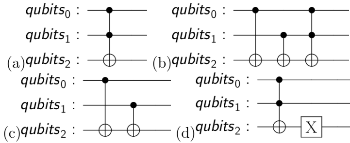
Figura 17 – Circuitos que representam as portas clássicas: (a) AND; (b) OR; (c) XOR e (d) NAND.
