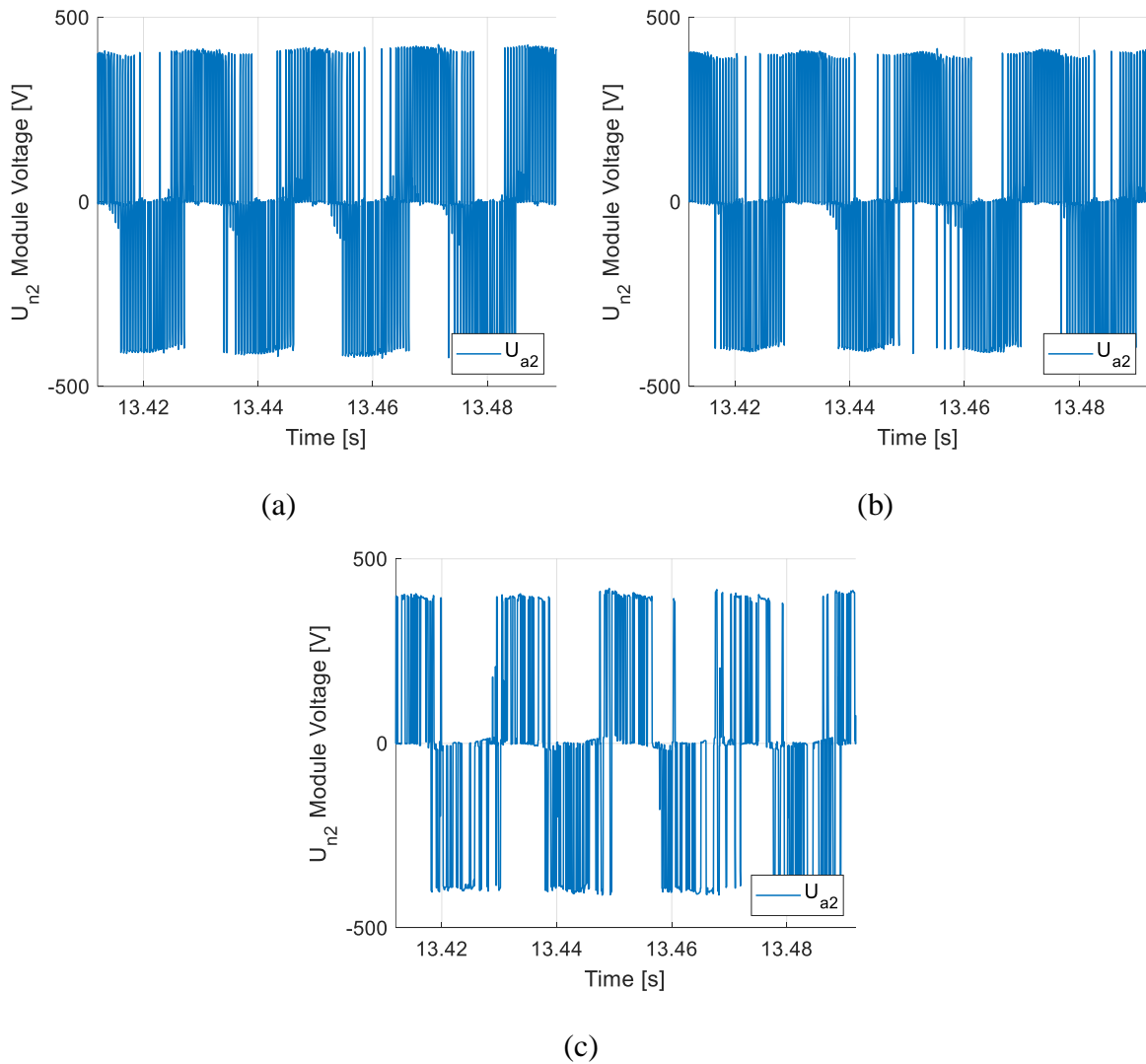
Figure 5-12– Synthesized STATCOM voltage – upper module: (a) CHB (4,000 \mu F); (b) CHB (1,200 \mu F); (c) SDC-CHB (1,200 \mu F) [7].
