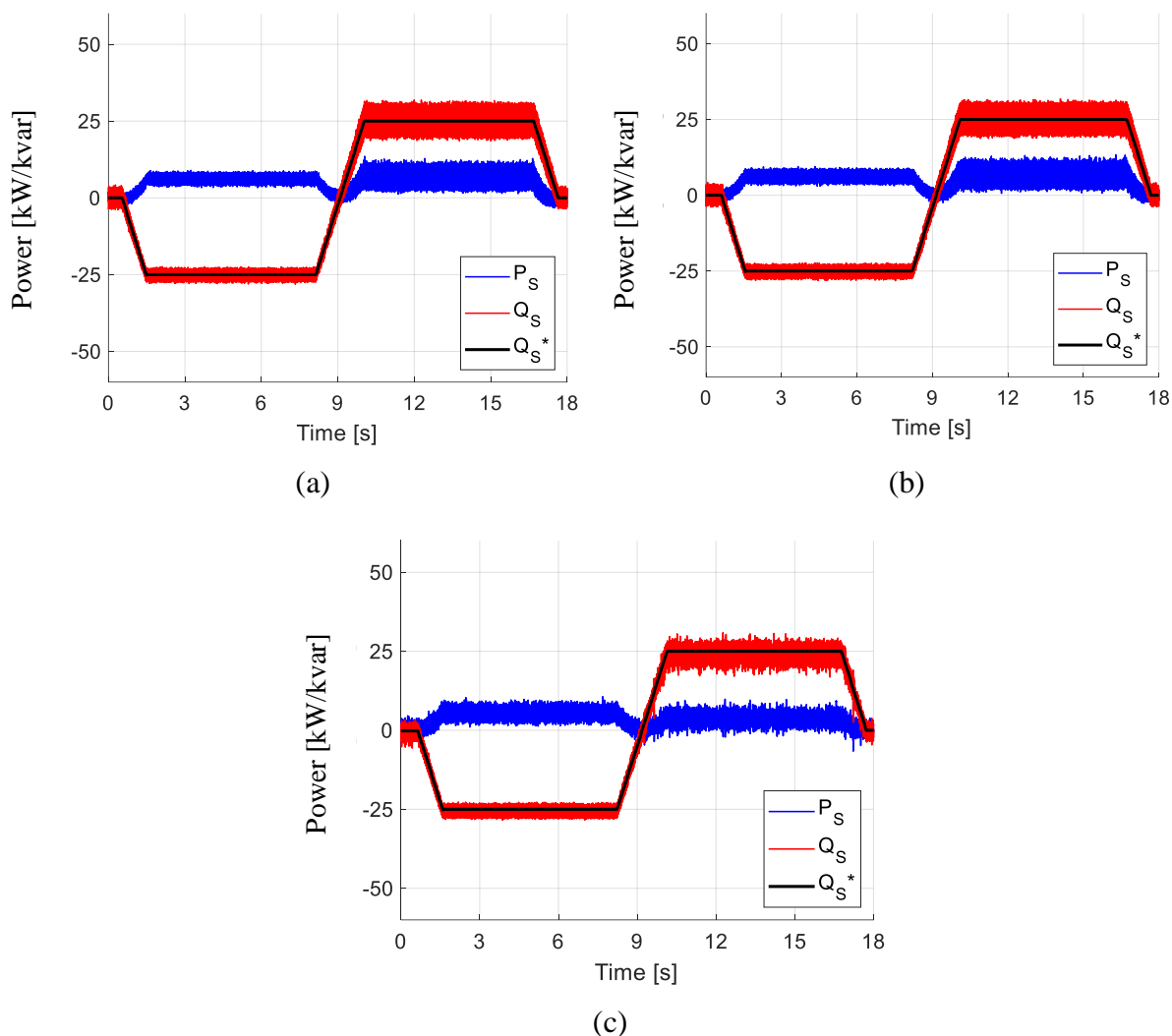
Figure 5-3– Active and reactive power: (a) CHB ( 4,000\mu F ); (b) CHB ( 1,200\mu F ); (c) SDC-CHB ( 1,200\mu F ) [7].
