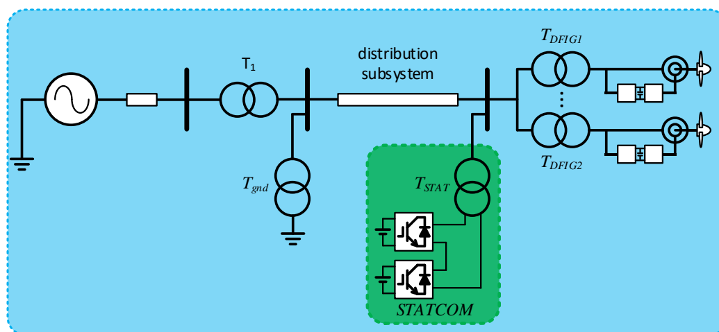
Figure 1-1– STATCOM application in a wind farm system.
