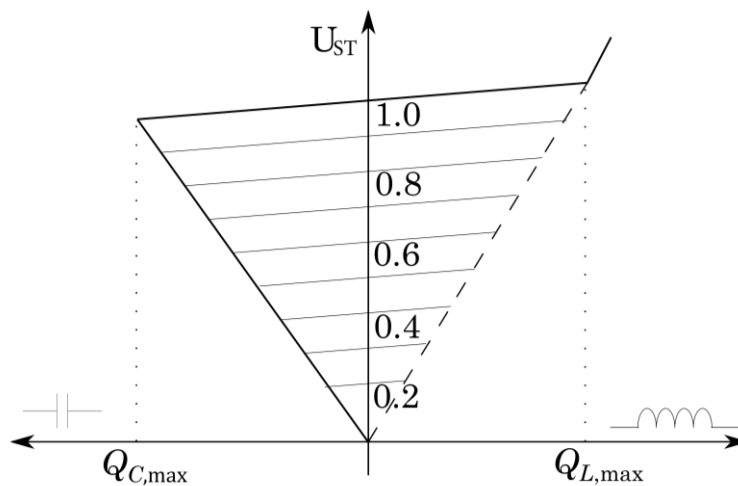
Figure 4-7– STATCOM U – Q Characteristics [97, 100]
