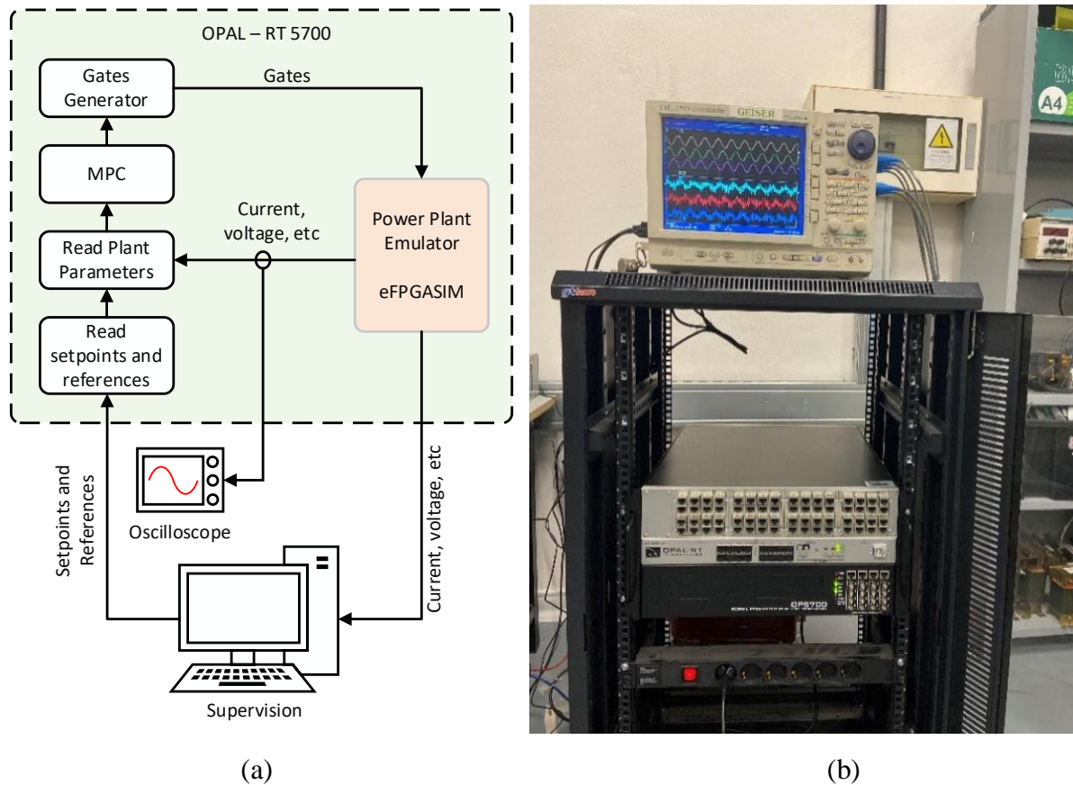
Figure 5-1– Hardware-In-the-Loop implementation: (a) OPAL-RT 5700 Flowchart; (b) Implementation image with emphasis on signals in the oscilloscope [7].
