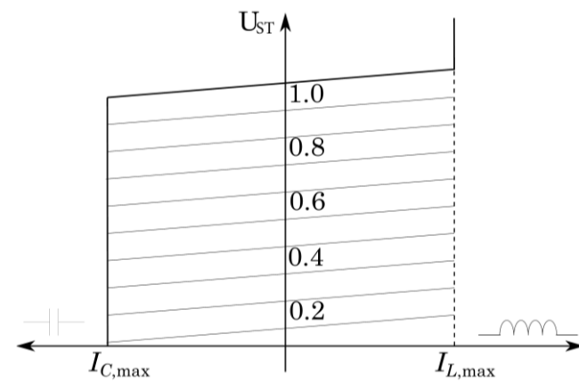
Figure 4-6– STATCOM U – I Characteristics [97, 98, 99]
