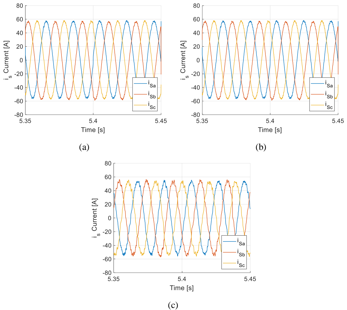
Figure 5-5– Three-phase grid currents: (a) CHB (4,000 \mu F ); (b) CHB(1,200 \mu F ); (c) SDC-CHB (1,200 \mu F ) [7].
