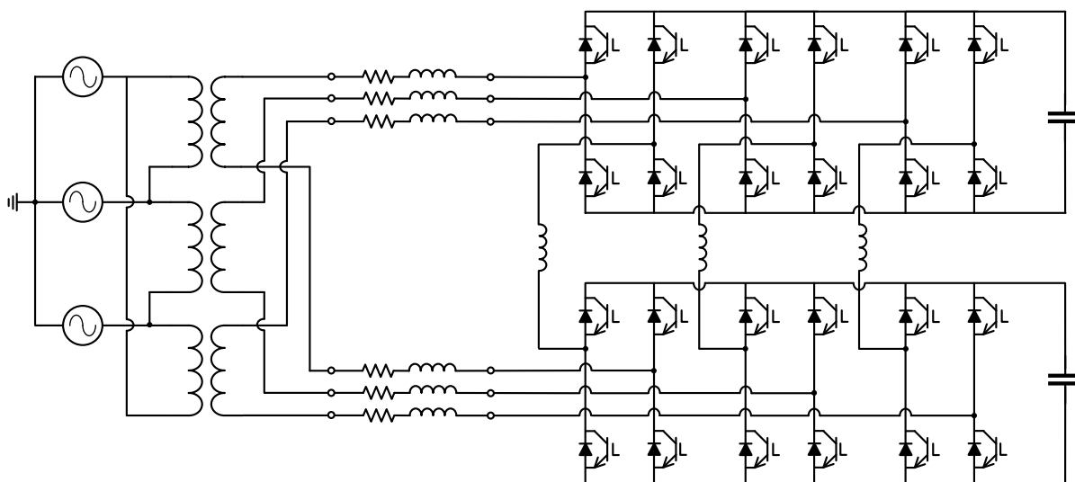
Figure 3-5– SDC-CHB STATCOM [7, 11].
