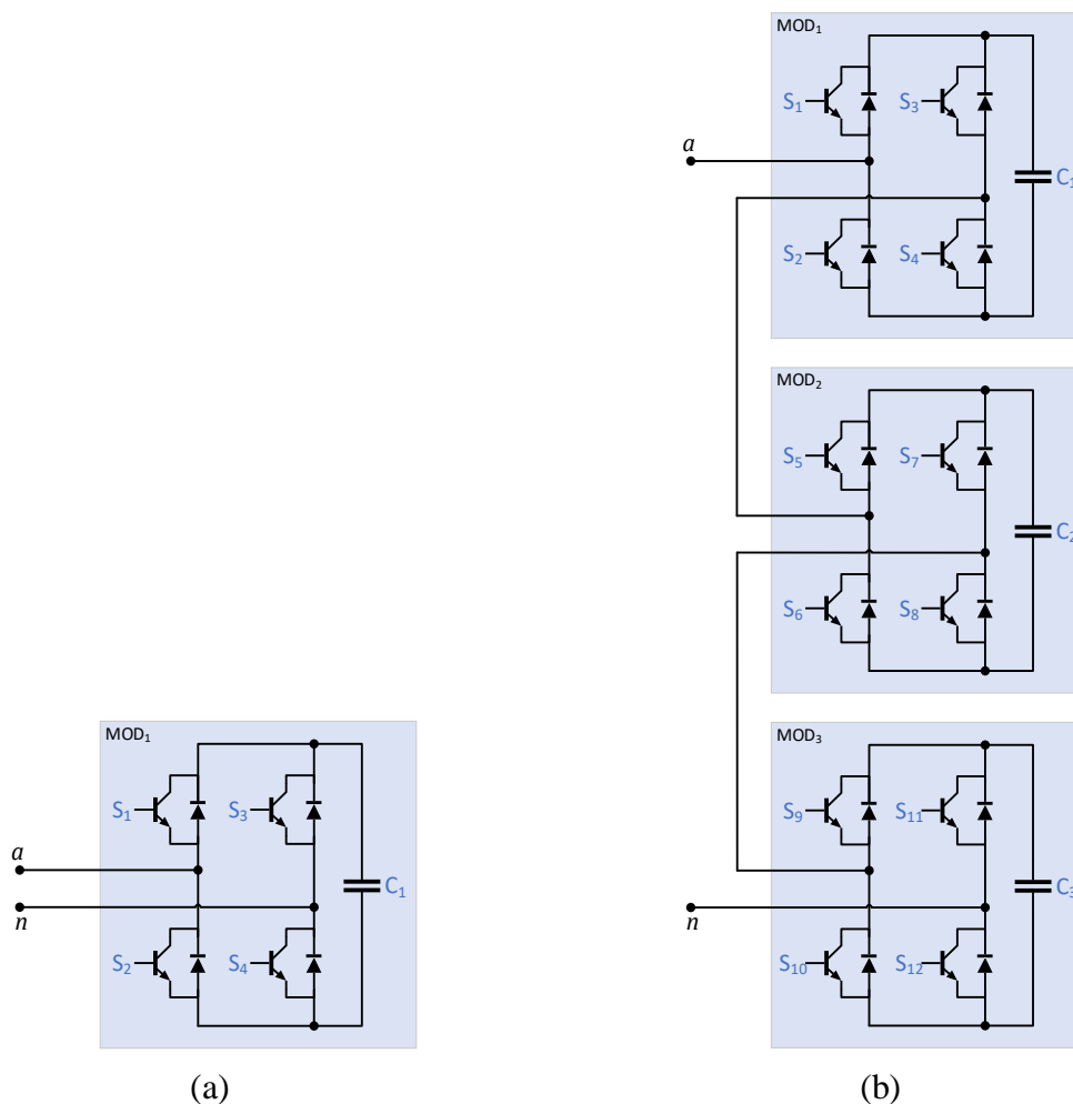
Figure 2-4– Contrast between the number of components of (a) a three-level CHB and (b) a seven-level CHB [3, 29, 30]
