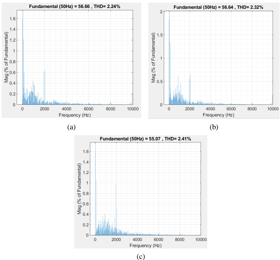
Figure 5-6– Grid current harmonic spectrum in inductive mode: (a) CHB (4,000 \mu F ); (b) CHB (1,200 \mu F ); (c) SDC-CHB (1,200 \mu F ) [7].
